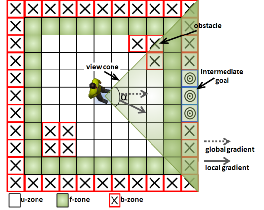
Figure 5: Agent Local Map. The update ( u -zone), free ( f -zone) and border zones ( b -zone) are shown. Blue and red cells correspond to the intermediate goal and obstacles, respectively.
